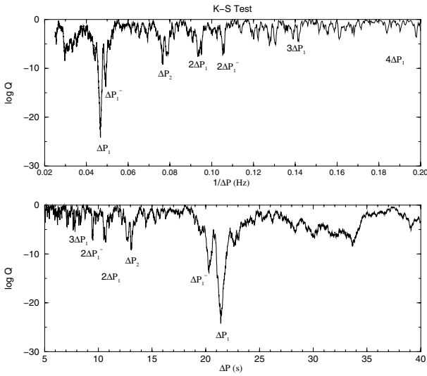
Fig. 5. The K-S applied to list of candidate pulsation periods.
