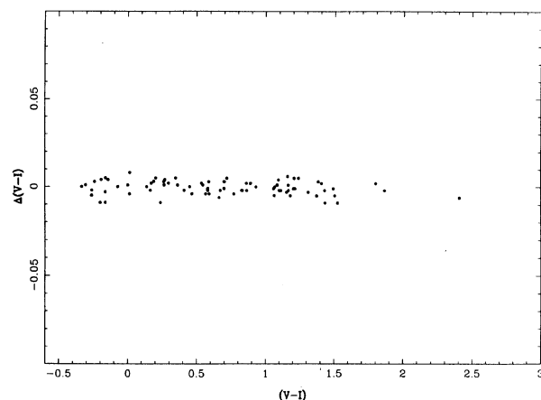
FIG. 24. A comparison of the (V-I) color index for the 81 standard star subset after all nonlinearity and transformation relations have been applied, as a function of Landolt's (1983) equatorial standard star's (V-I) color index.
