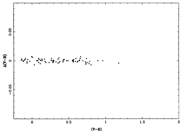
FIG. 22. A comparison of the (V-R) color index for the 81 standard star subset after all nonlinearity and transformation relations have been applied, as a function of Landolt's (1983) equatorial standard star's (V-R) color index.
