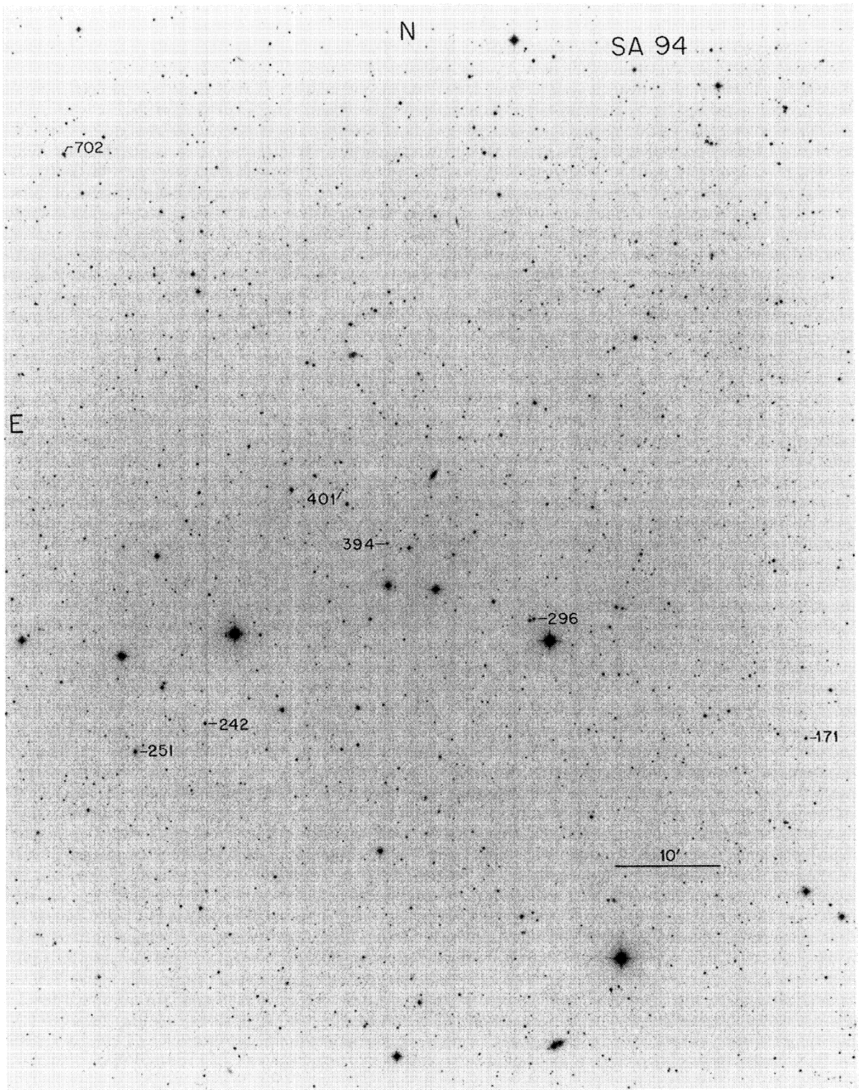
PLATE 28. The field of Selected Area 94.
