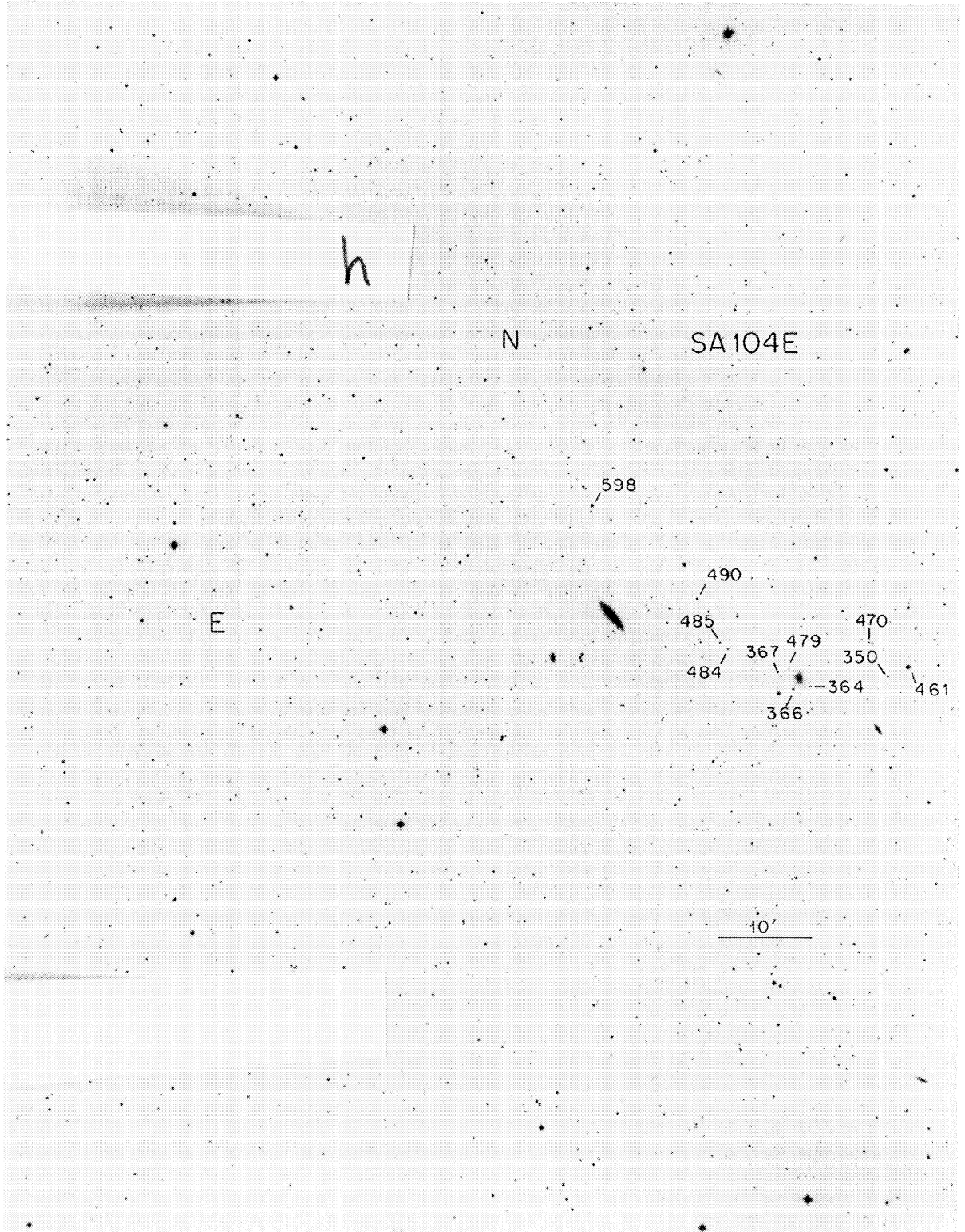
PLATE 49. The field of the eastern part of Selected Area 104.
