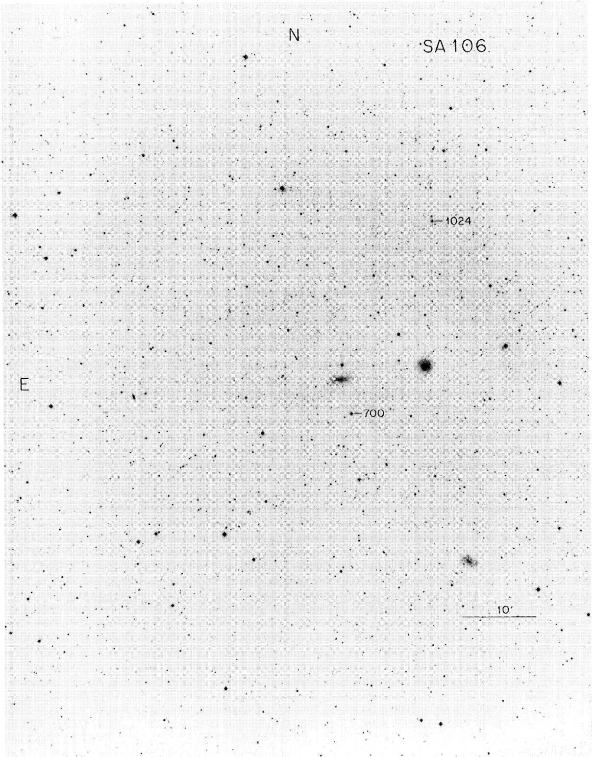
PLATE 54. The field of Selected Area 106.
