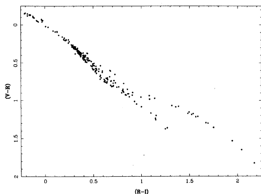
FIG. 39. The (V-R) , (R-I) color-color plot for the 217 new standard stars in Table 2.
