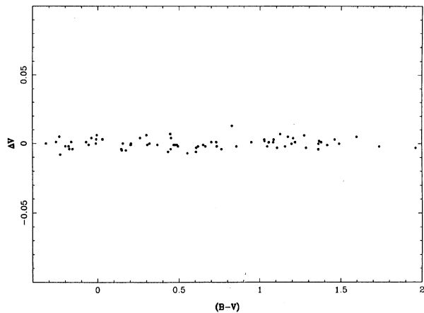
FIG. 7. A comparison of the V magnitude as obtained with serial No. N49701 RCA 31034A as a function of Landolt's (1983) standard star (B-V) color index.
