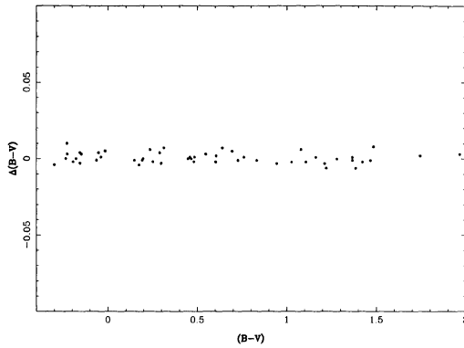
FIG. 41. A comparison of the (B-V) color indices obtained with the Hamamatsu R943-02 as a function of the (B-V) color indices obtained with the RCA 31034A.
