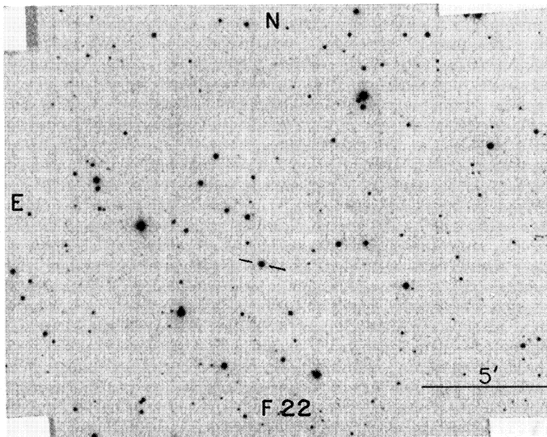
PLATE 26. (a) The field of the star PG 0220+132. (b) The field of the star Feige 22.
