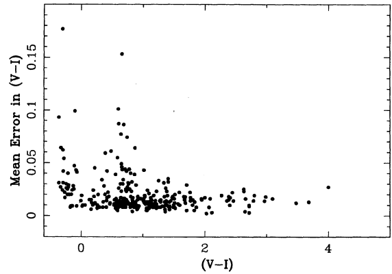
FIG. 35. The weighted mean error of a single observation in (V-I) for the 298 standard stars as a function of (V-I) .
