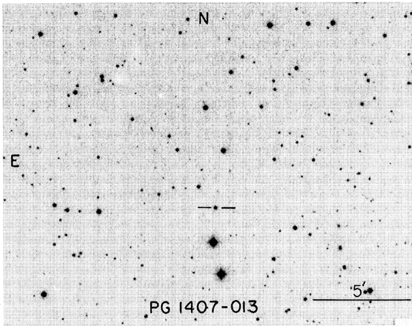
PLATE 53. (a) The field of the star HD 121968. (b) The field of the star PG 1407-013.
