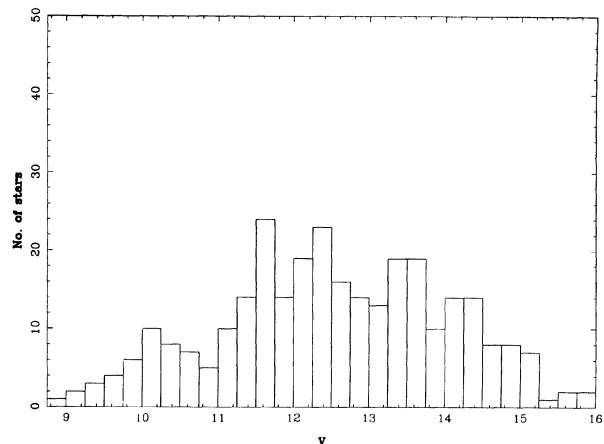
FIG. 25. The magnitude distribution for the 298 standard stars in intervals of 0.25V mag.
