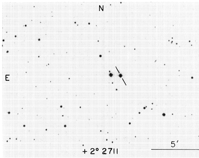
PLATE 52. (a) Sequence in the field of the star PG 1323-086. (b) The field of the star BD +2°2711.
