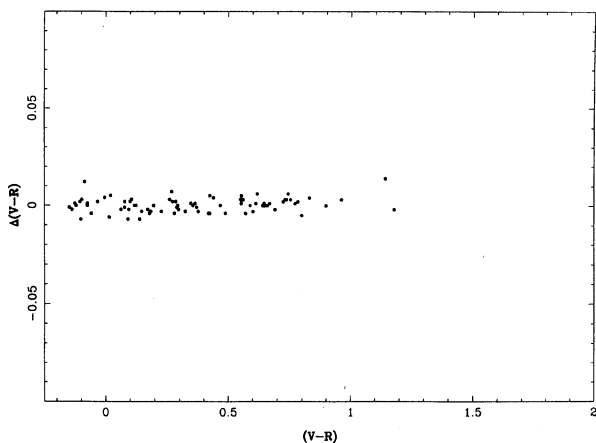
FIG. 16. A comparison of the (V-R) color indices obtained with the Hamamatsu R943-02 as a function of the transformed RCA (V-R) color index data.
