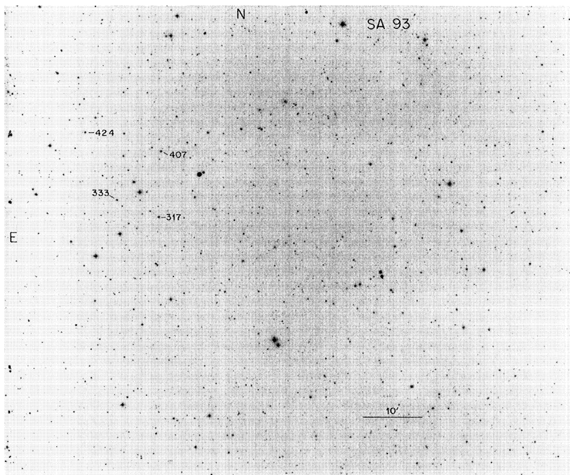
PLATE 24. The field of Selected Area 93.
