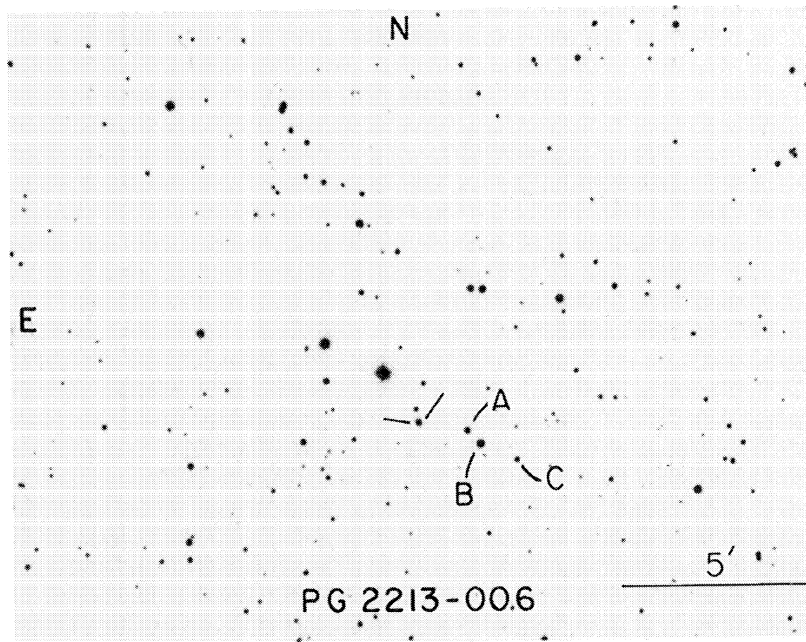
PLATE 70. (a) The field of the star G93 48. (b) Sequence in the field of the star PG 2213-006.
