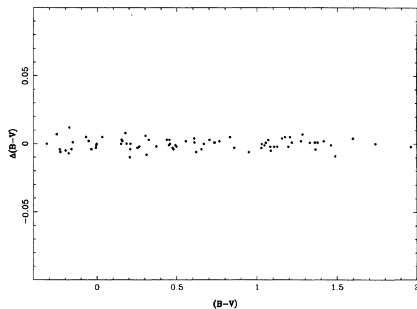
FIG. 20. A comparison of the (B-V) color index for the 81 standard star subset after all nonlinearity and transformation relations have been applied, as a function of Landolt's (1983) equatorial standard star's (B-V) color index.
