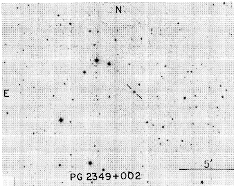
PLATE 75. (a) Sequence in the field of the star PG 2336+004. (b) The field of the star PG 2349+002.
