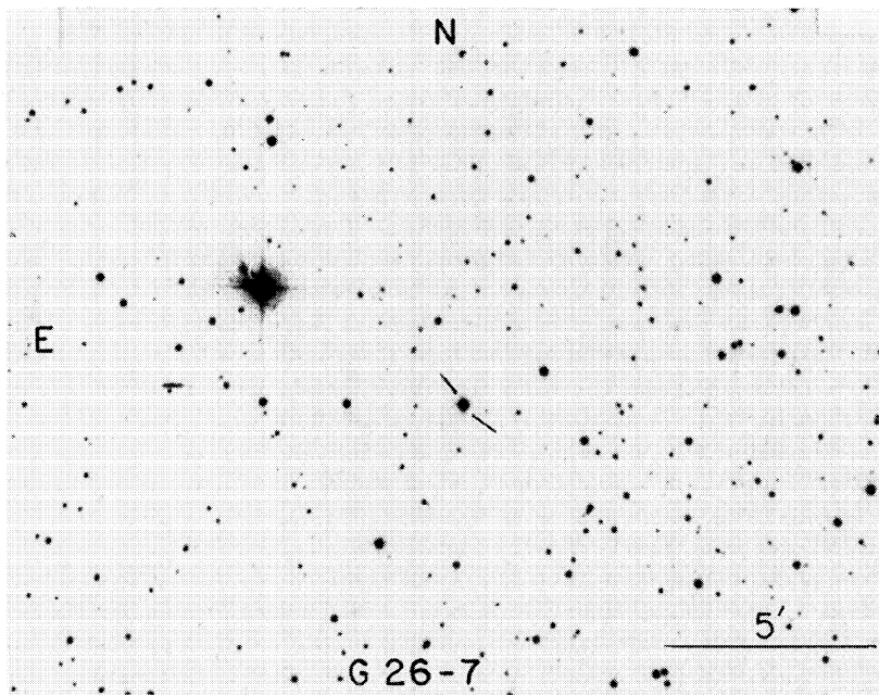
PLATE 68. (a) The field of the star Wolf 918. (b) The field of the star G26 7.
