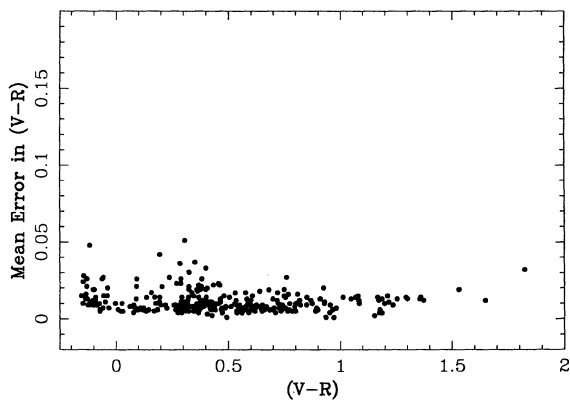
FIG. 33. The weighted mean error of a single observation in (V-R) for the 298 standard stars as a function of (V-R) .
