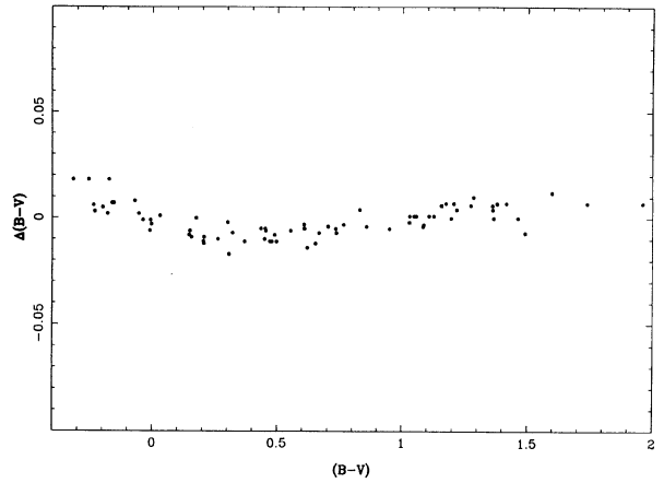
FIG. 8. A comparison of the (B-V) color index as obtained with serial No. N49701 RCA 31034A as a function of Landolt's (1983) standard star (B-V) color index.
