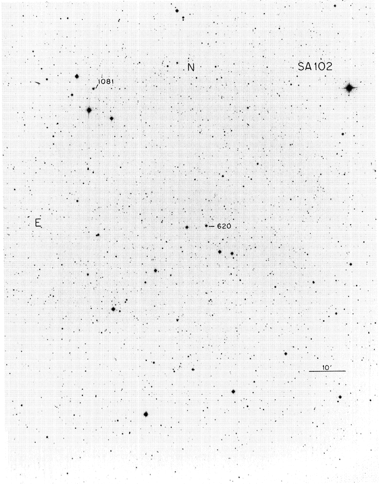
PLATE 44. The field of Selected Area 102.
