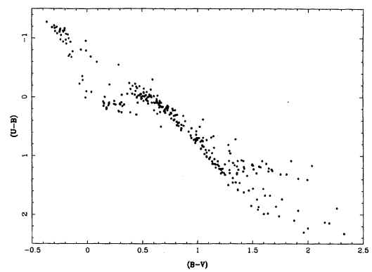
FIG. 36. The (U-B) , (B-V) color-color plot for the 298 standard stars in Table 2.
