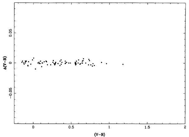
FIG. 10. A comparison of the (V-R) color index as obtained with serial No. N49701 RCA 31034A as a function of Landolt's (1983) standard star (V-R) color index.
