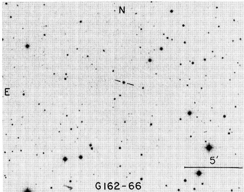
PLATE 41. (a) The field of the star G44 27. (b) The field of the star G162 66.
