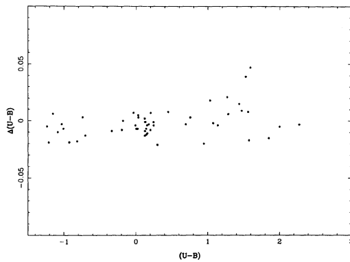
FIG. 42. A comparison of the (U-B) color indices obtained with the Hamamatsu R943-02 as a function of the (U-B) color indices obtained with the RCA 31034A.
