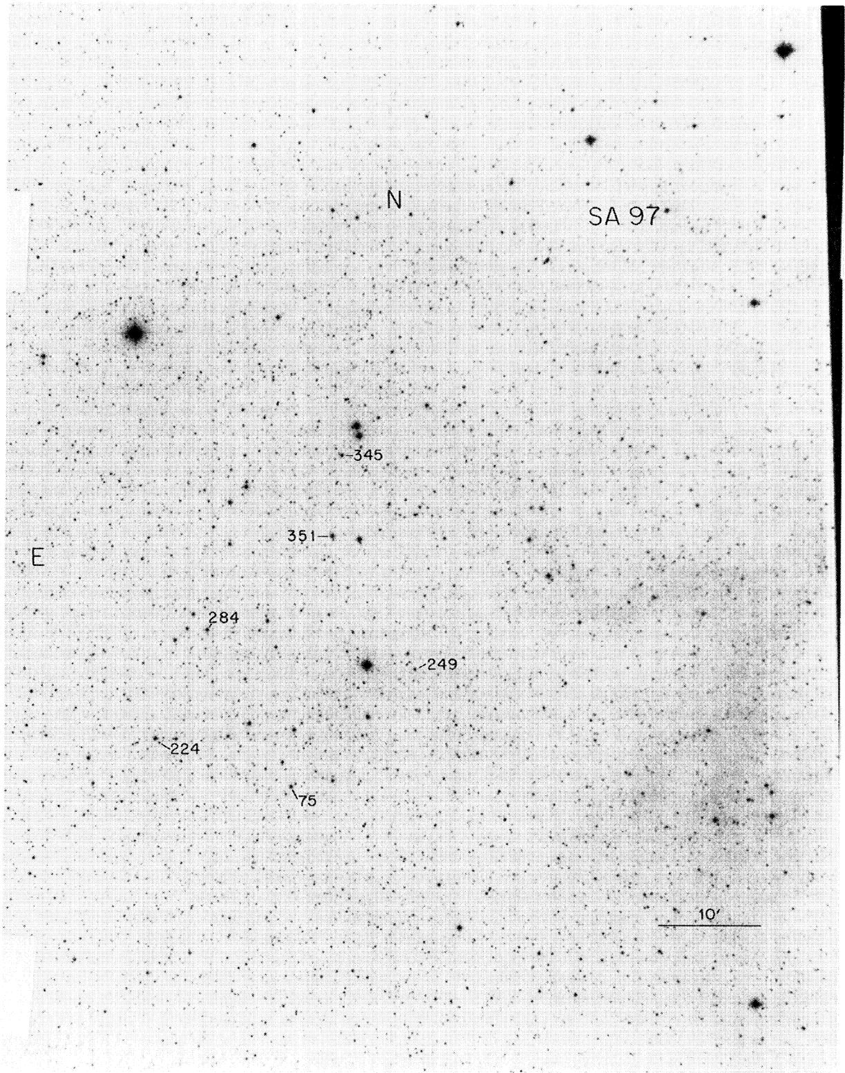
PLATE 33. The field of Selected Area 97.
