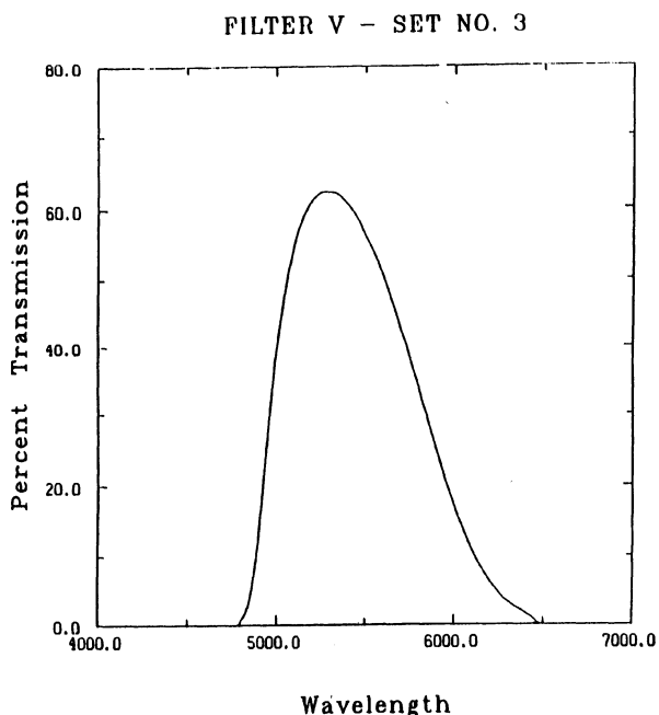
FIG. 46. The transmission characteristics of the V filter: 2 mm GG495 + 2 mm BG 18.
