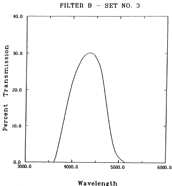
FIG. 47. The transmission characteristics of the B filter: 2 mm GG385 + 2 mm BG 18 + 2 mm BG 12.
