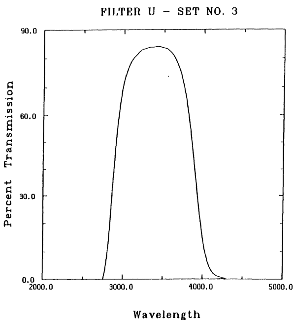
FIG. 48. The transmission characteristics of the U filter: Corning 9863 + solid CuSO_4 crystal.
