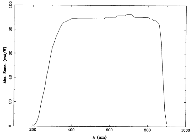
FIG. 53. The average absolute sensitivity as a function of wavelength for several RCA 31034A photomultipliers.
