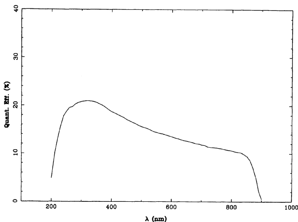
FIG. 52. The quantum efficiency as a function of wavelength for RCA 3103A, serial No. N49701.
