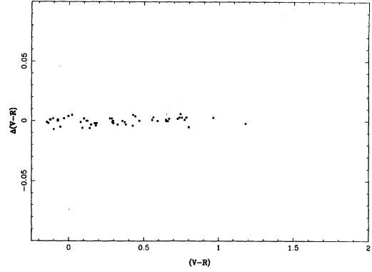
FIG. 43. A comparison of the (V-R) color indices obtained with the Hamamatsu R943-02 as a function of the (V-R) color indices obtained with the RCA 31034A.
