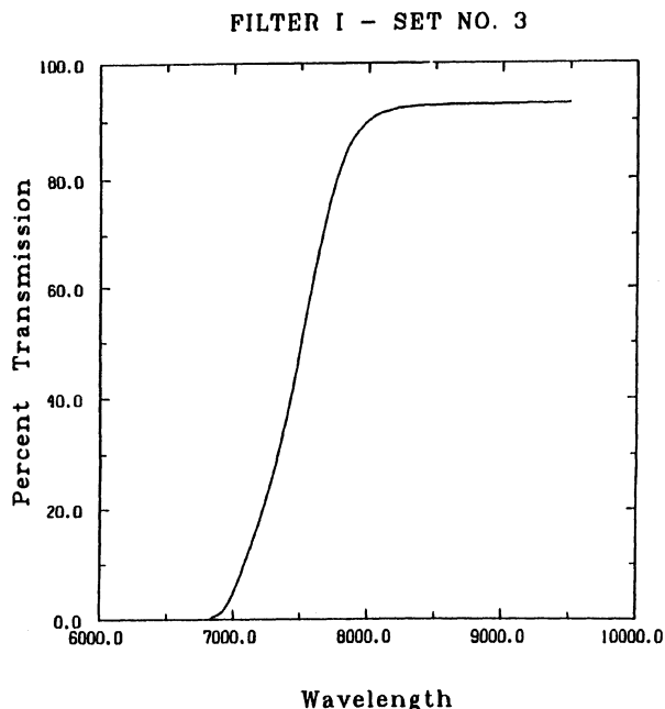
FIG. 50. The transmission characteristics of the I filter: 3 mm RG 715+1 mm RG 780.
