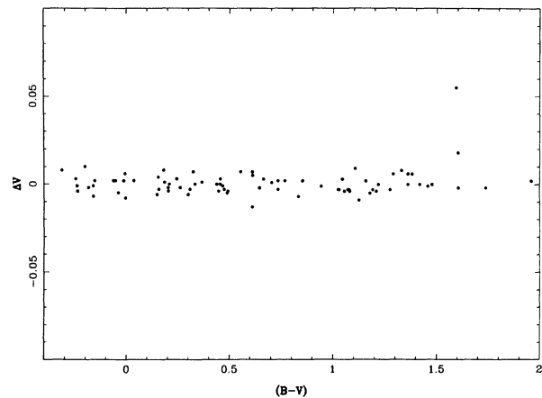
FIG. 13. A comparison of the V magnitudes obtained with the Hamamatsu R943-02 as a function of the transformed RCA (B-V) color index data.
