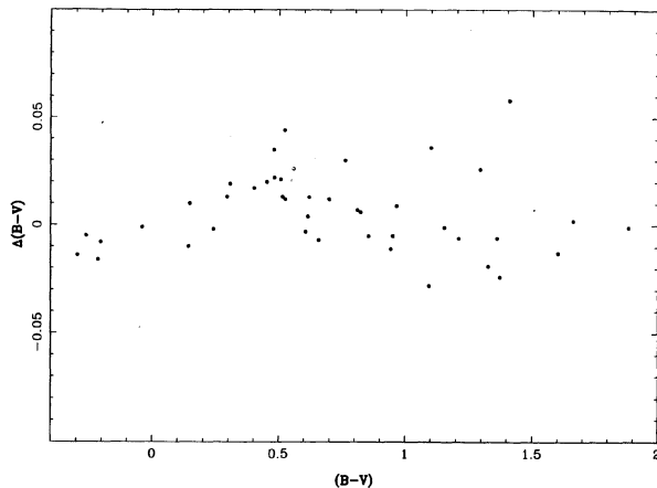
FIG. 2. A comparison of the ( B-V ) color index as determined with filter set one as a function of filter set two's ( B-V ) color index.
