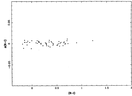
FIG. 44. A comparison of the (R-I) color indices obtained with the Hamamatsu R943-02 as a function of the (R-I) color indices obtained with the RCA 31034A.
