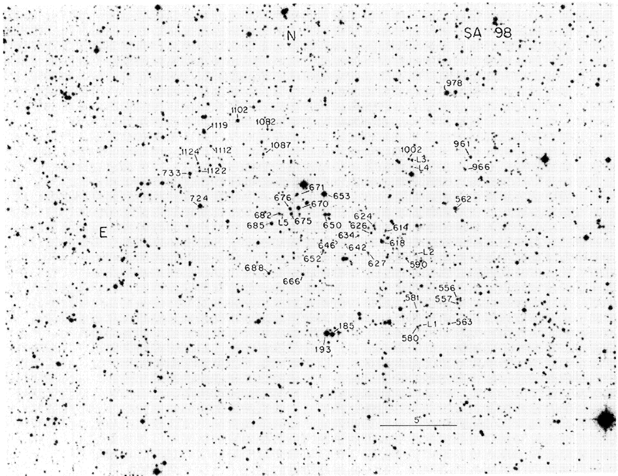
PLATE 34. The field of Selected Area 98.
