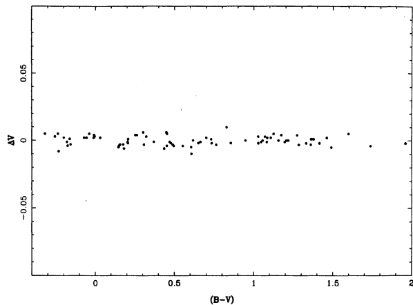
FIG. 19. A comparison of the V magnitude for the 81 standard star subset after all nonlinearity and transformation relations have been applied, as a function of Landolt's (1983) equatorial standard star's (B-V) color index.
