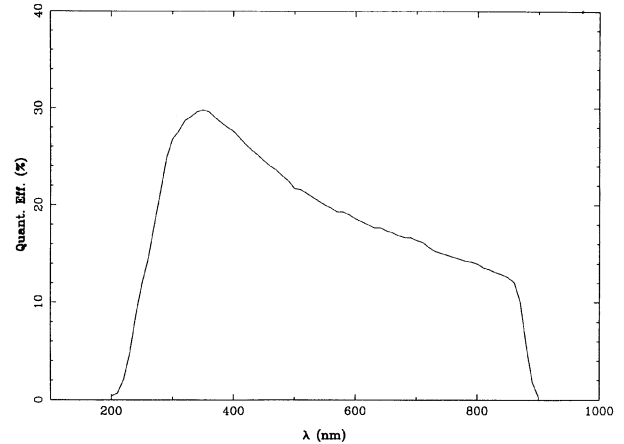
FIG. 54. The average quantum efficiency as a function of wavelength for several RCA 31034A photomultipliers.
