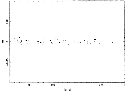
FIG. 40. A comparison of the V magnitudes obtained with the Hamamatsu R943-02 as a function of the (B-V) color index obtained with the RCA 31034A.
