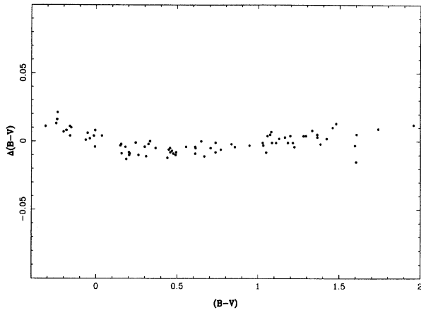
FIG. 14. A comparison of the (B-V) color indices obtained with the Hamamatsu R943-02 as a function of the transformed RCA (B-V) color index data.
