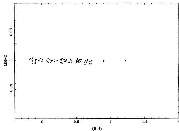
FIG. 23. A comparison of the (R-I) color index for the 81 standard star subset after all nonlinearity and transformation relations have been applied, as a function of Landolt's (1983) equatorial standard star's (R-I) color index.
