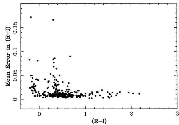
FIG. 34. The weighted mean error of a single observation in (R-I) for the 298 standard stars as a function of (R-I) .
