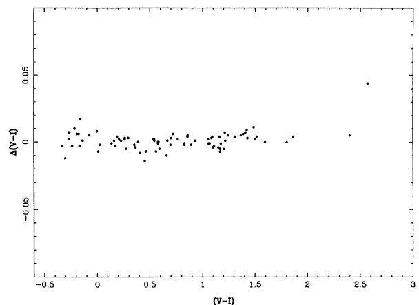
FIG. 18. A comparison of the (V-I) color indices obtained with the Hamamatsu R943-02 as a function of the transformed RCA (V-I) color index data.
