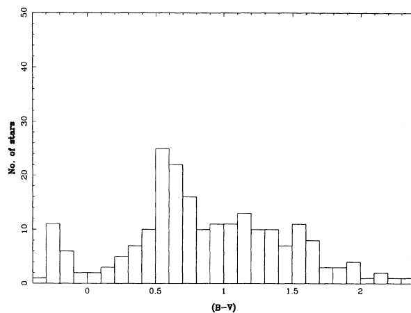
FIG. 28. The distribution in the (B-V) color index for the 217 new standard stars in intervals of 0.1 mag.
