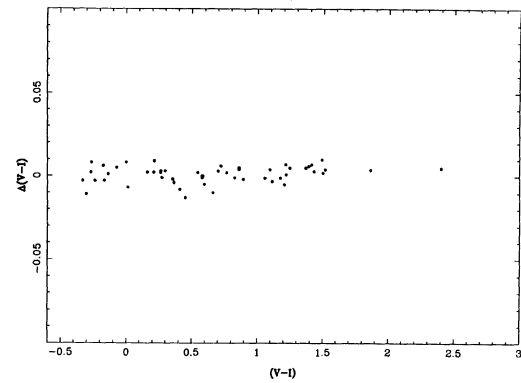
FIG. 45. A comparison of the (V-I) color indices obtained with the Hamamatsu R943-02 as a function of the (V-I) color indices obtained with the RCA 31034A.
