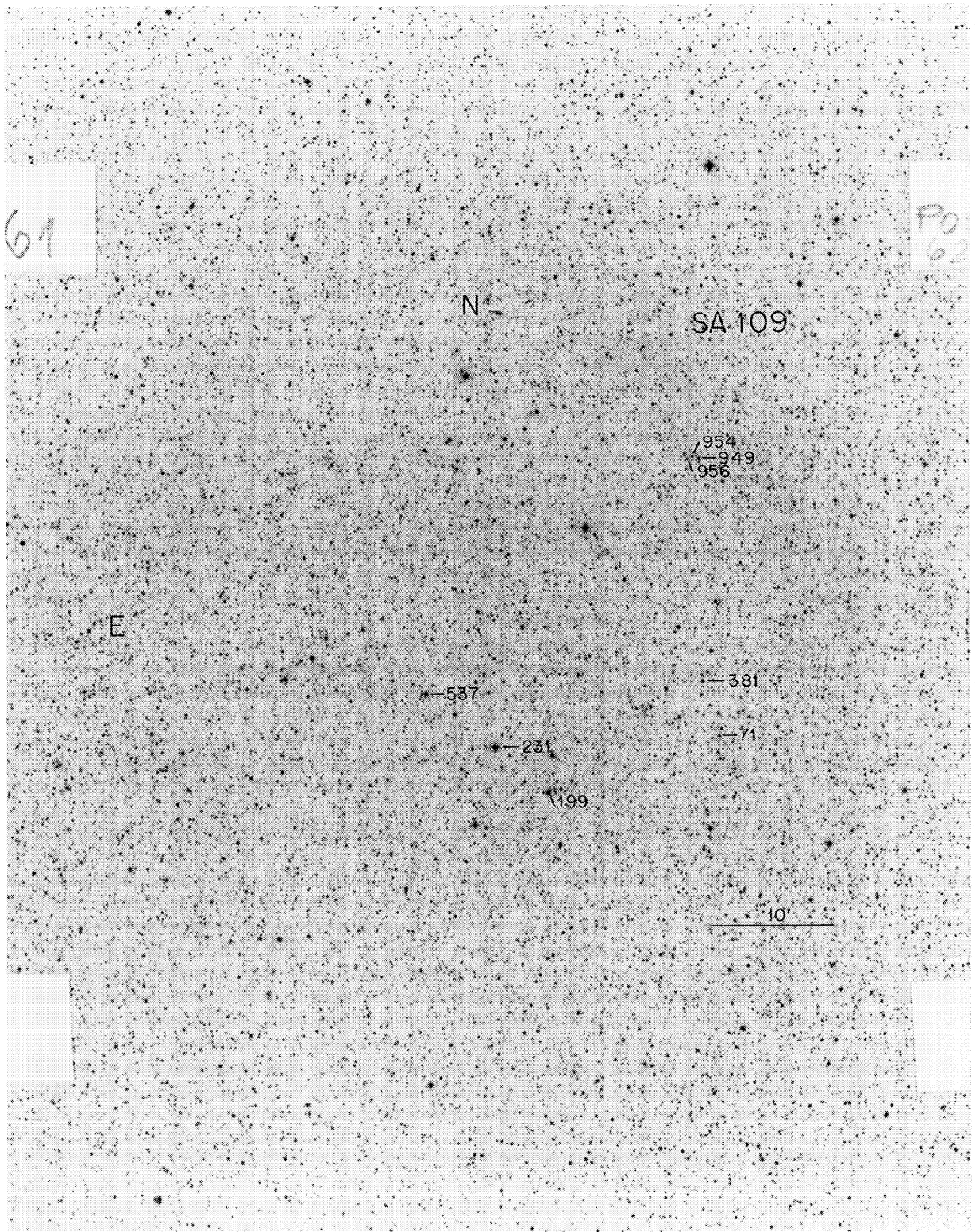
PLATE 63. The field of Selected Area 109.
