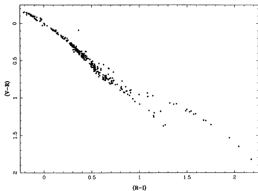
FIG. 38. The (V-R) , (R-I) color-color plot for the 298 standard stars in Table 2.
