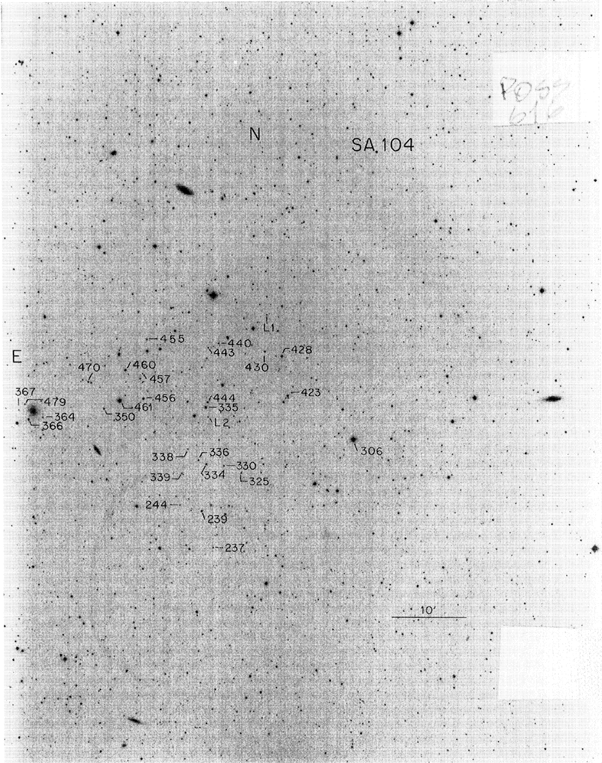
PLATE 48. The field of Selected Area 104.
