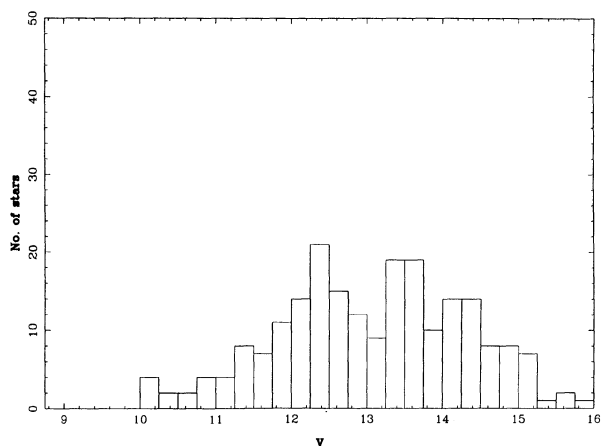
FIG. 26. The magnitude distribution for the 217 new standard stars in intervals of 0.25V mag.
